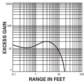
Polarized Reflex (3 in diameter retroreflector)
