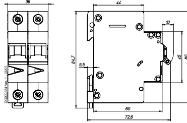
1+N-poles, 2-poles
