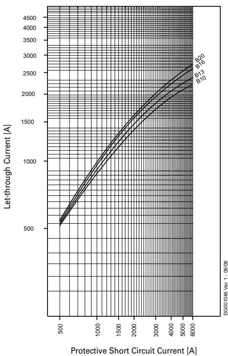
Characteristic B
