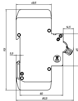
2-poles without rotary handle
