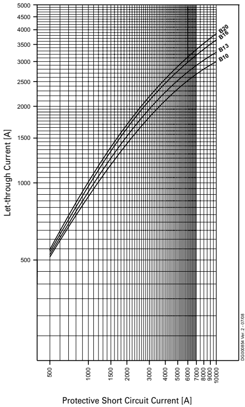
Characteristic B
