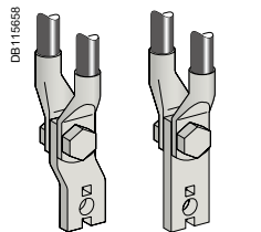
Mounting detail: 2 cables with lugs.
