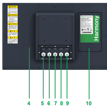
19" rear view
