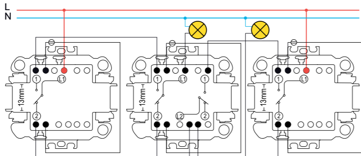
2 two-way switches + 1 double two-way switches
