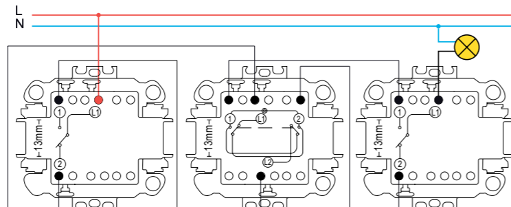
2 two-way switches + 1 intermediate switch with locator lamp
