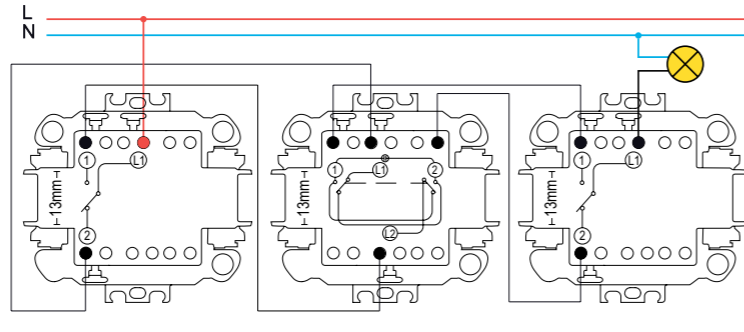
2 two-way switches or 2 two-way switches with locator lamp + 1 intermediate switch
